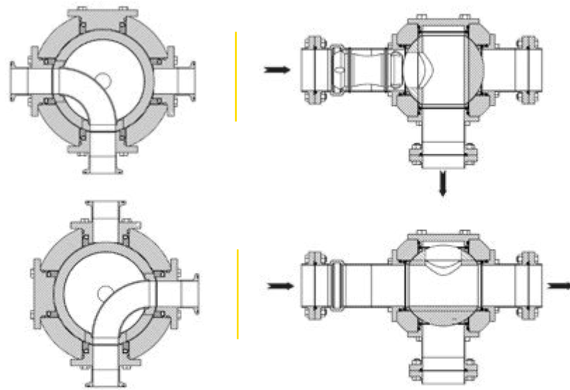
3-Way L-Port Valve
